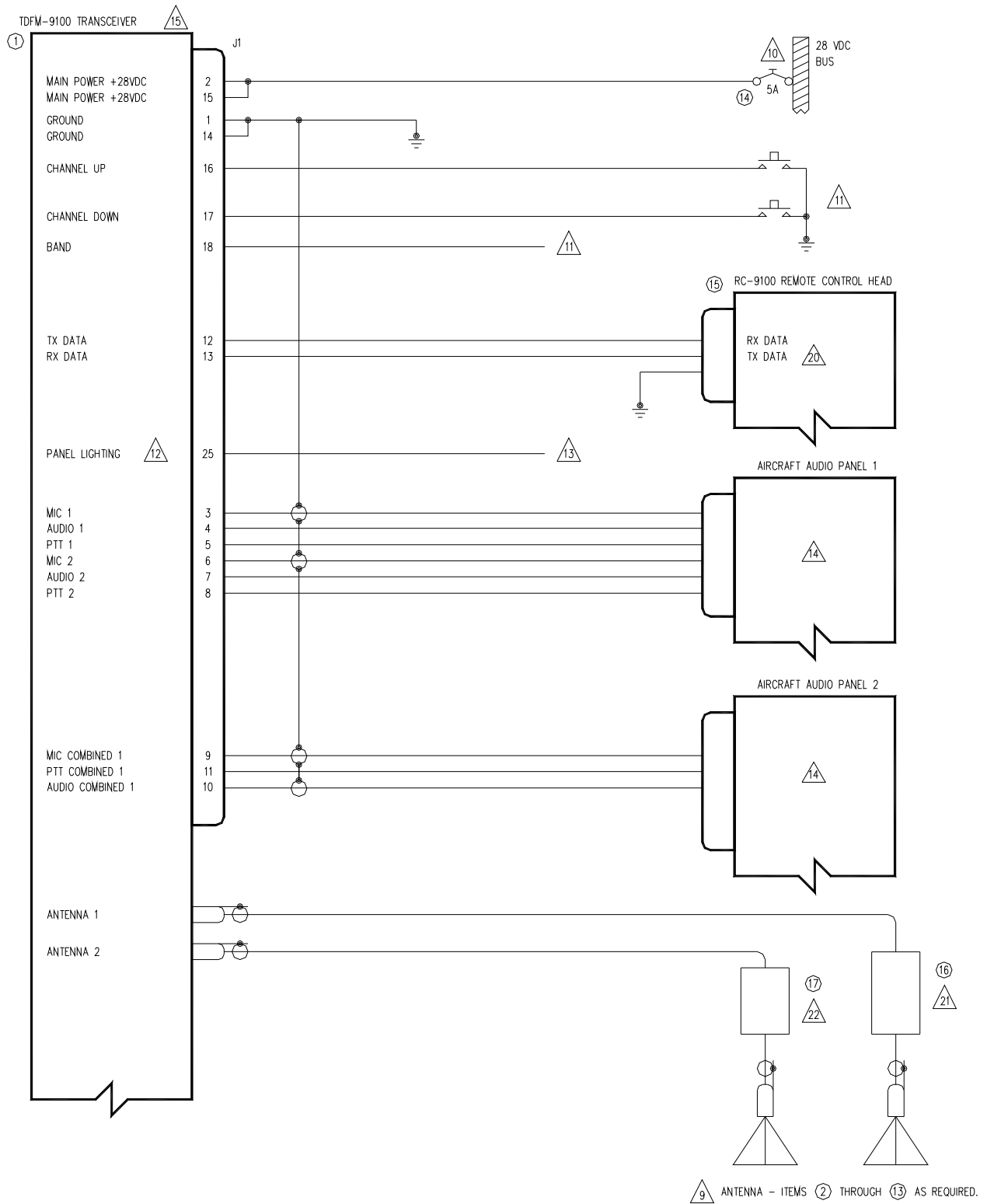
FIGURE 6: Wiring Connections for Separate and Combined Band Control
