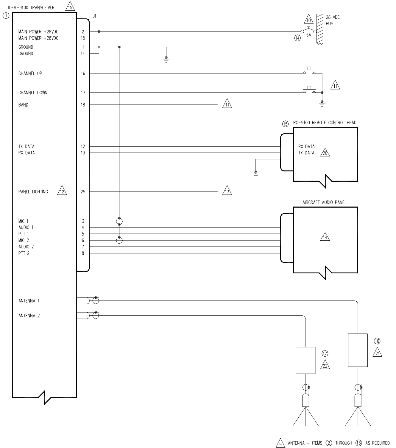
FIGURE 4: Wiring Connections for Separate Band Control
