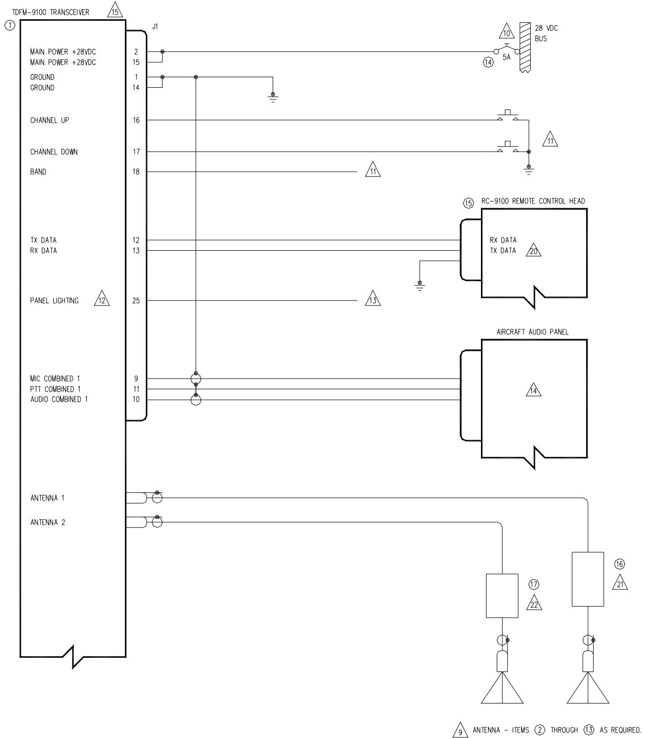
FIGURE 5: Wiring Connections for Combined Band Control
